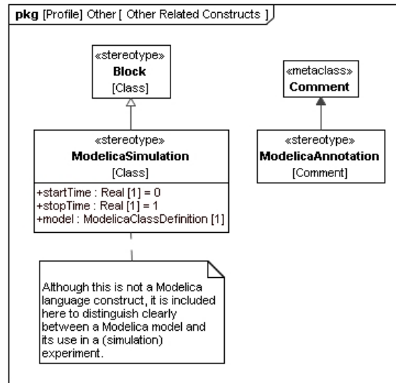
Figure 12: Package diagram with definitions of Modelica-related constructs
