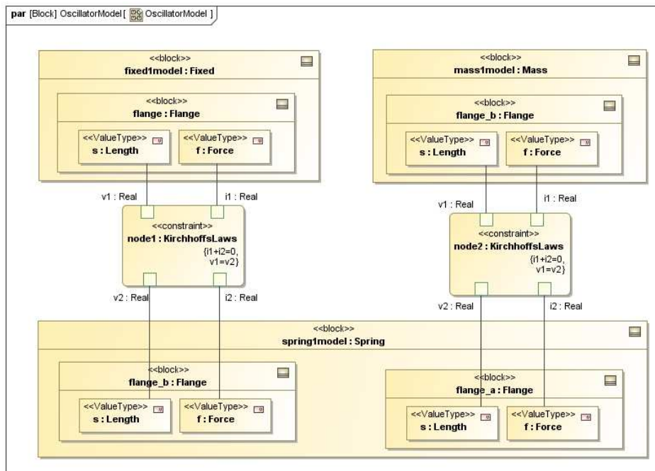
Figure 18: Mass-Spring model as represented in a Parametric Diagram.
