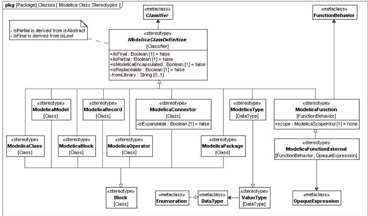
Figure 5: Package diagram with an overview of the stereotypes for Modelica Classes
