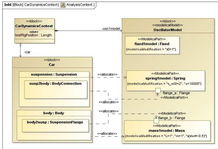
Figure 19: The Block Definition Diagram for the Analysis Context of the continuous dynamics analysis.
