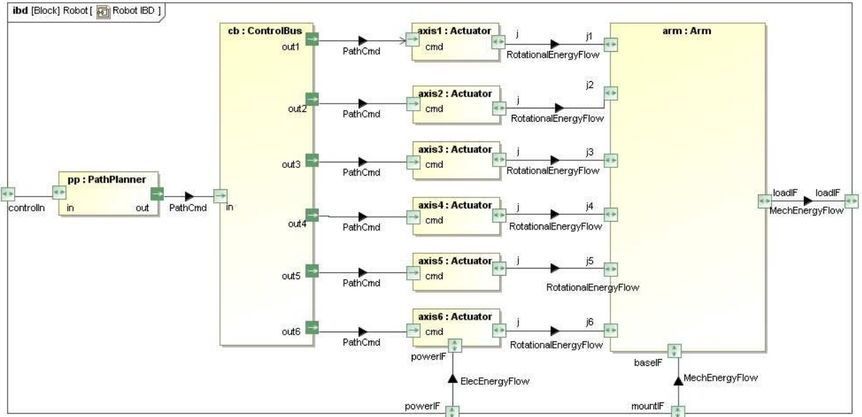
Figure 27: The internal block diagram for the robot, illustrating its decomposition into the path planner, the control bus, the actuators and the mechanical structure of the robot arm.
