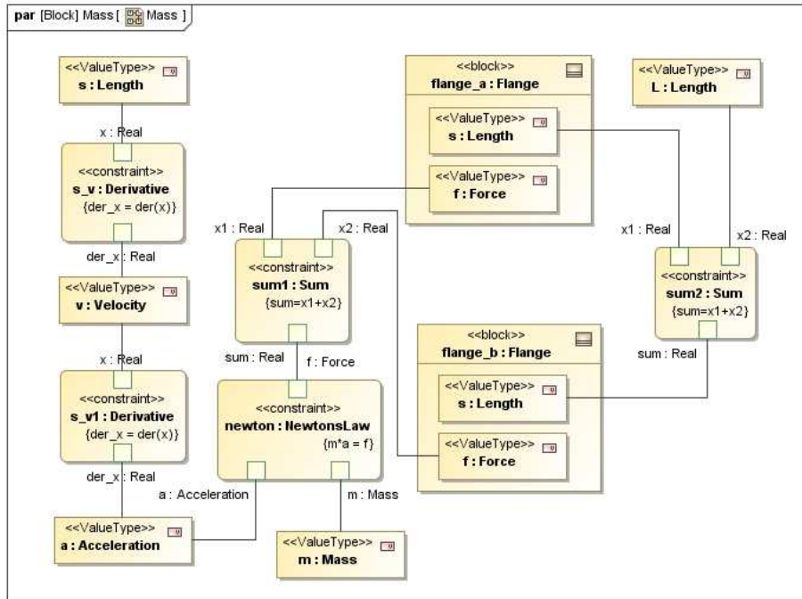
Figure 17: Mass model as it could be represented in a Parametric Diagram.
