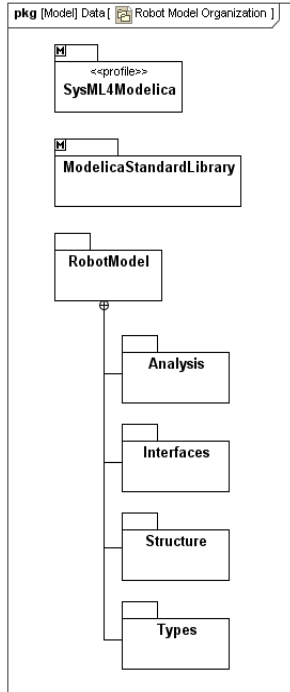
Figure 22: The package organization of the robot model.
