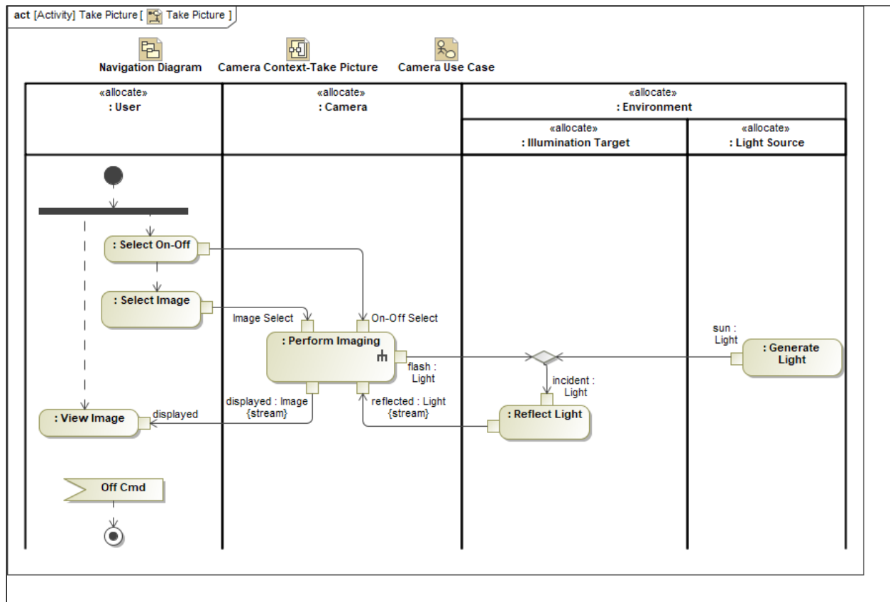
Figure 3.12. Top Level Behavior - Take Picture
