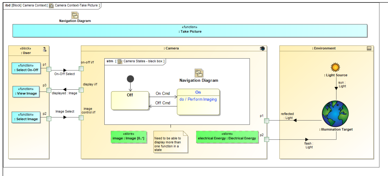
Figure 3.14. Camera Context with State Machine
