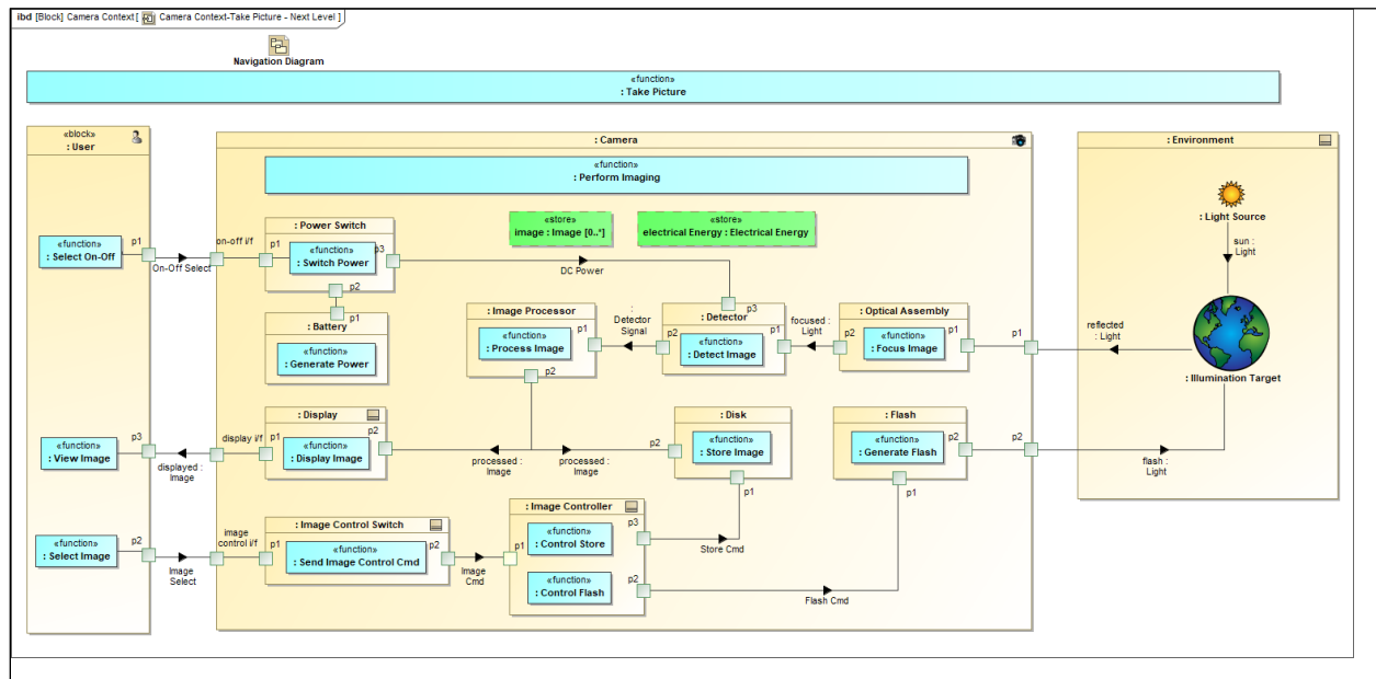
Figure 3.13. Camera Context with Take Picture Functions
