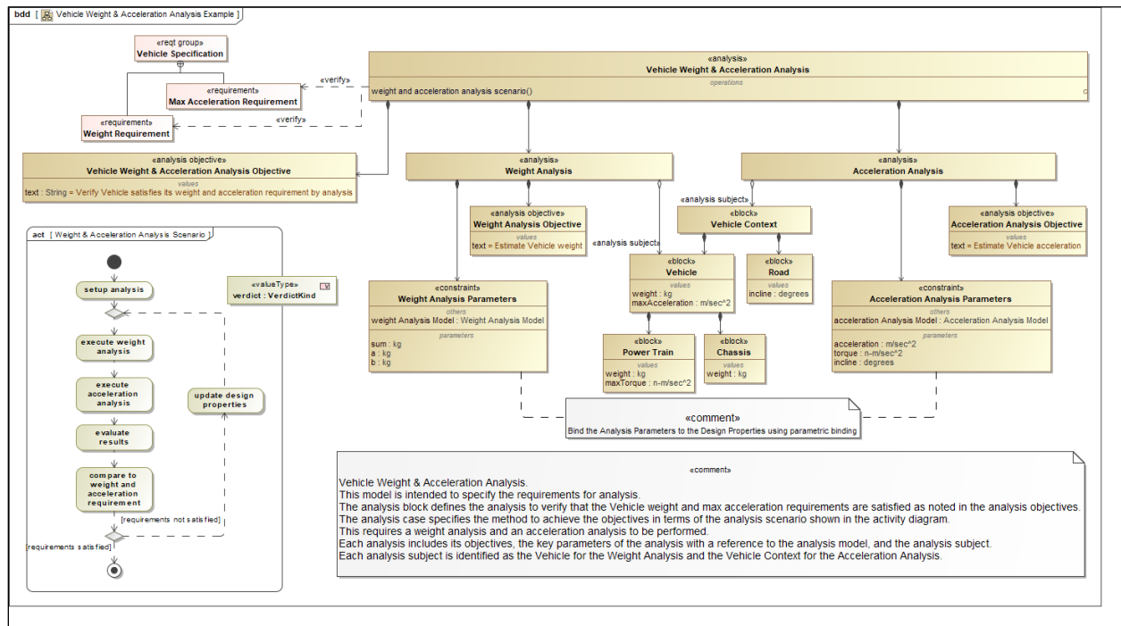
Figure 3.20. Vehicle Weight & Acceleration Analysis
