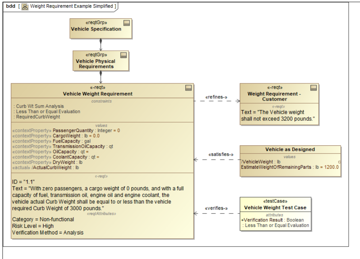
Figure 3.16. Example Weight Requirement
