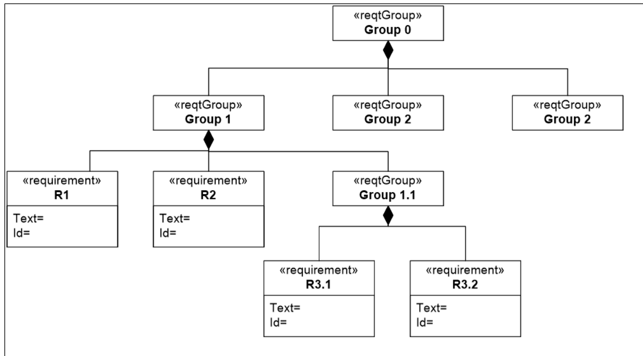
Figure 3.15. Requirement Groups
