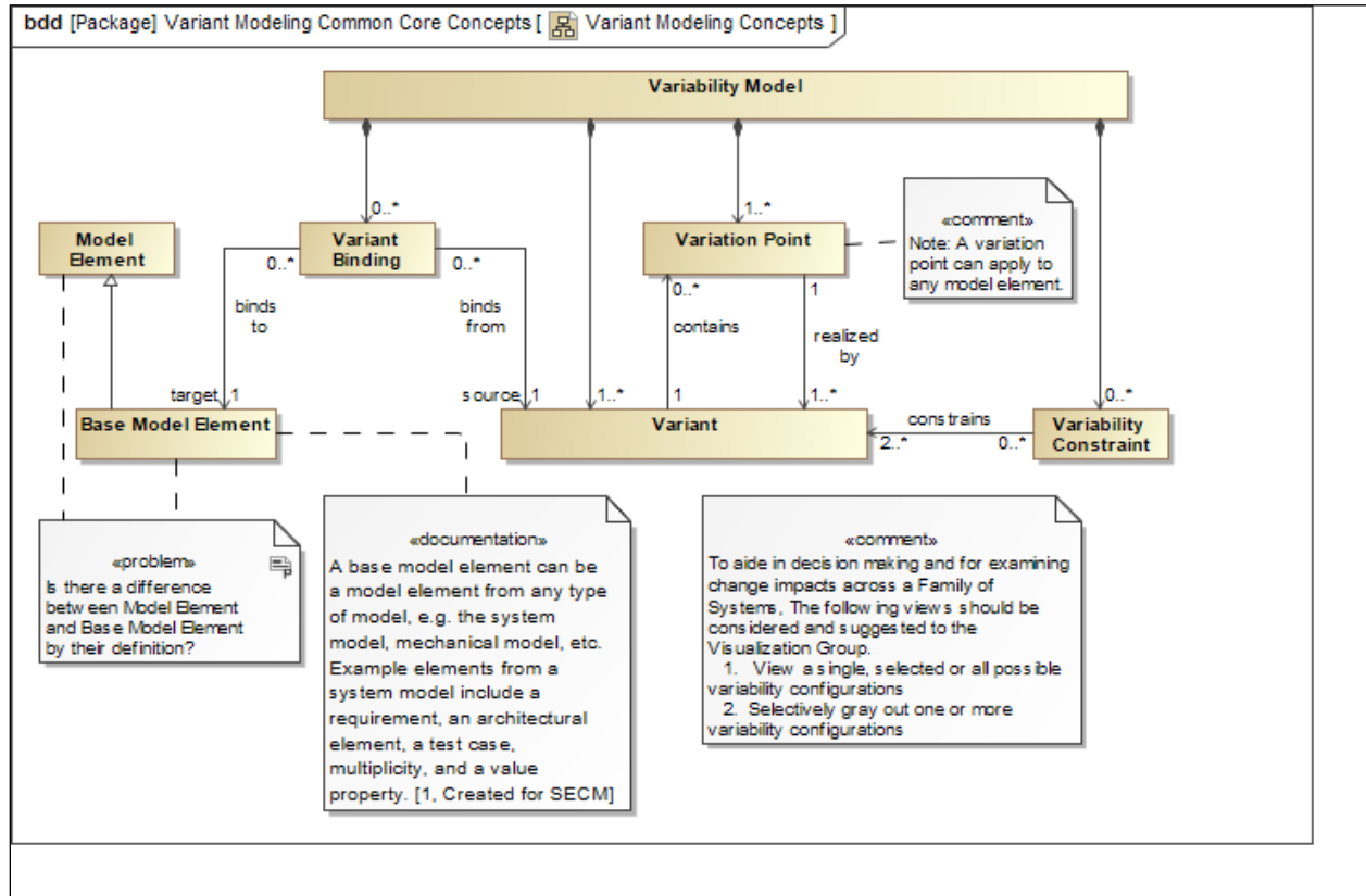
Figure 3.7. Variability Concepts
