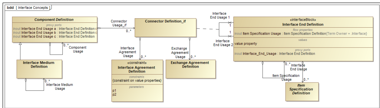
Figure 3.11. Interface Concepts
