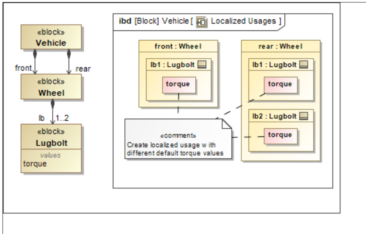
Figure 3.8. Specifying an unambiguous system design configuration
