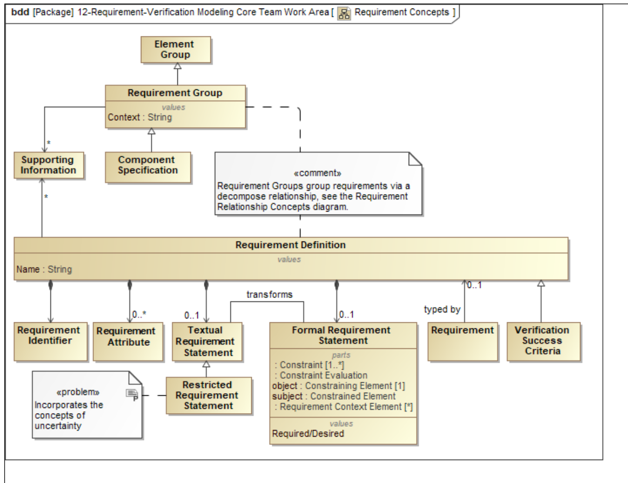
Figure 3.17. Requirement Concepts
