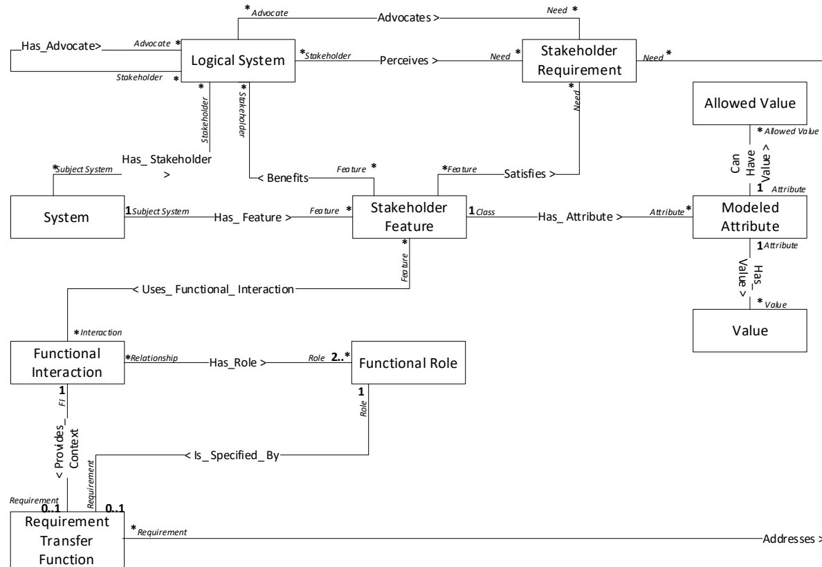
Figure 4: Feature Framework View
