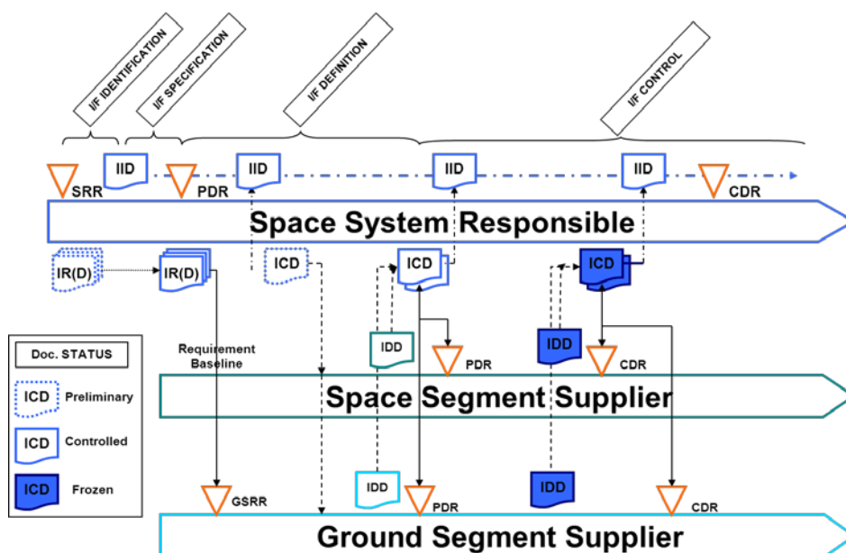
Figure 4-5: Typical space to ground segment interface life cycle
