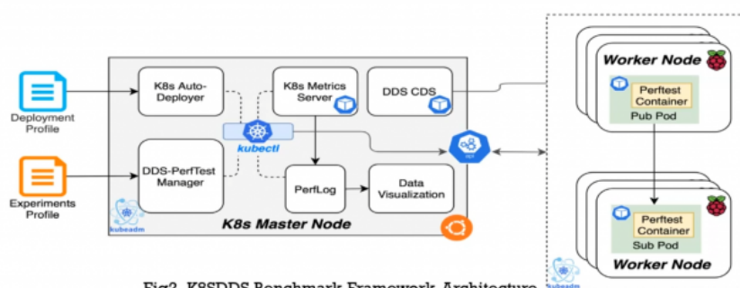
Fig2. K8SDDS Benchmark Framework Architecture
