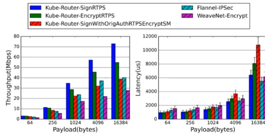
Fig7. Performance comparison of security implementations on application-layer(DDS Security plugin) and network-layer(Flannel-IPSec,WeaveNet-Encrypt). Communication pattern: 1pub-1sub . Reliability: enabled, Batching: disabled. Test period: 120 seconds.
