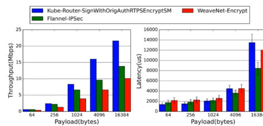
Fig8. Performance comparison of security implementations on application-layer(DDS Security plugin) and network-layer(Flannel-IPSec,WeaveNet-Encrypt) in multi-subscriber use case. Communication pattern: 1pub-4sub . Reliability: enabled, Batching: disabled. Test period: 120 seconds.
