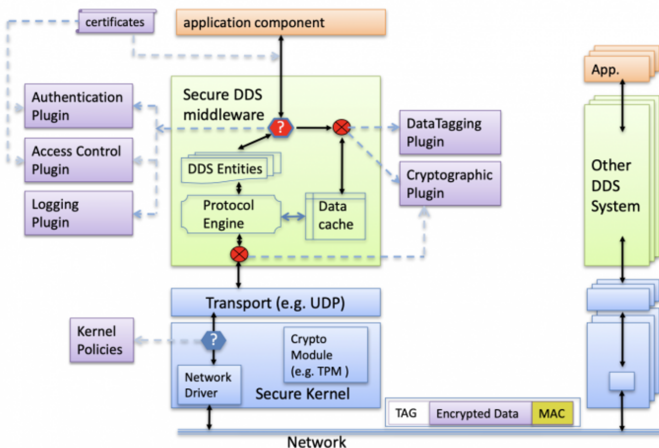
Figure 1: Overall architecture for Data Distribution Service (DDS) Security
