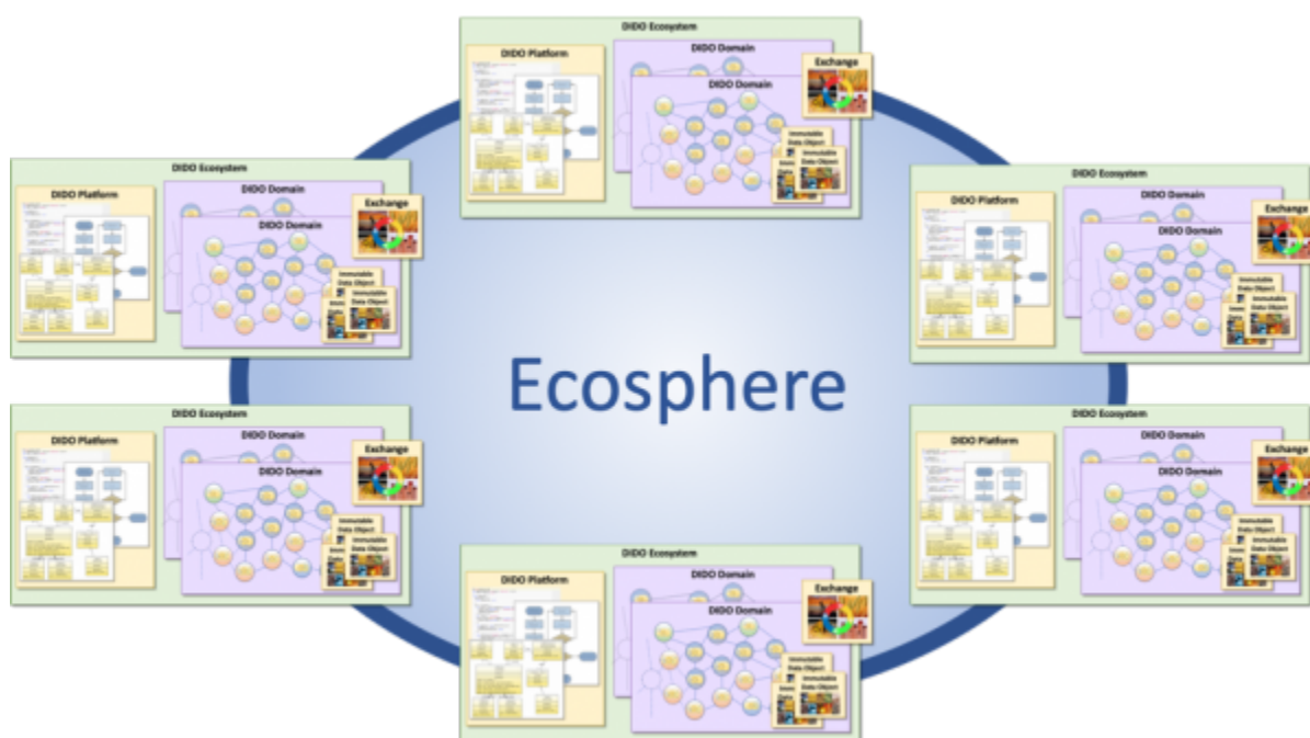
Figure 1: Ecosphere
