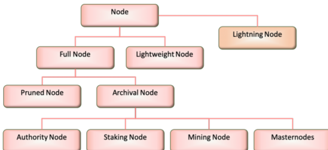
Figure 3: DIDO Node Taxonomy: Node Types
