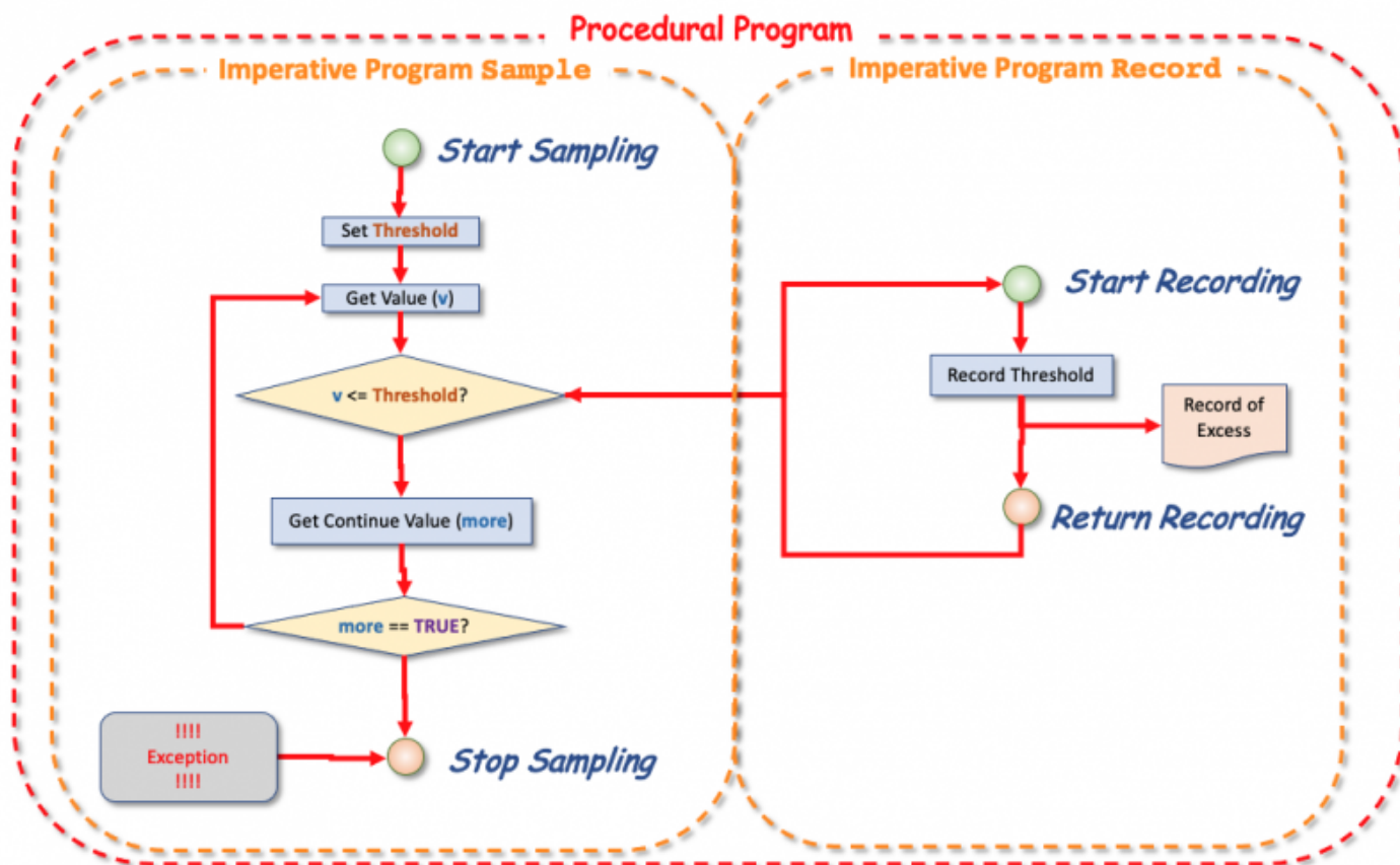
Figure 4: The difference between Imperative and Procedural Programming.
