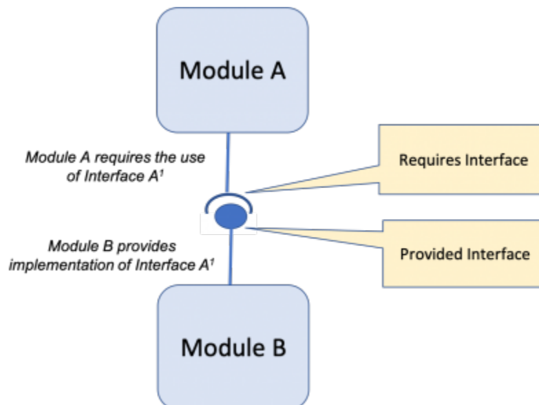
Figure 1: Modeling Modules Provided and Required Interfaces.
