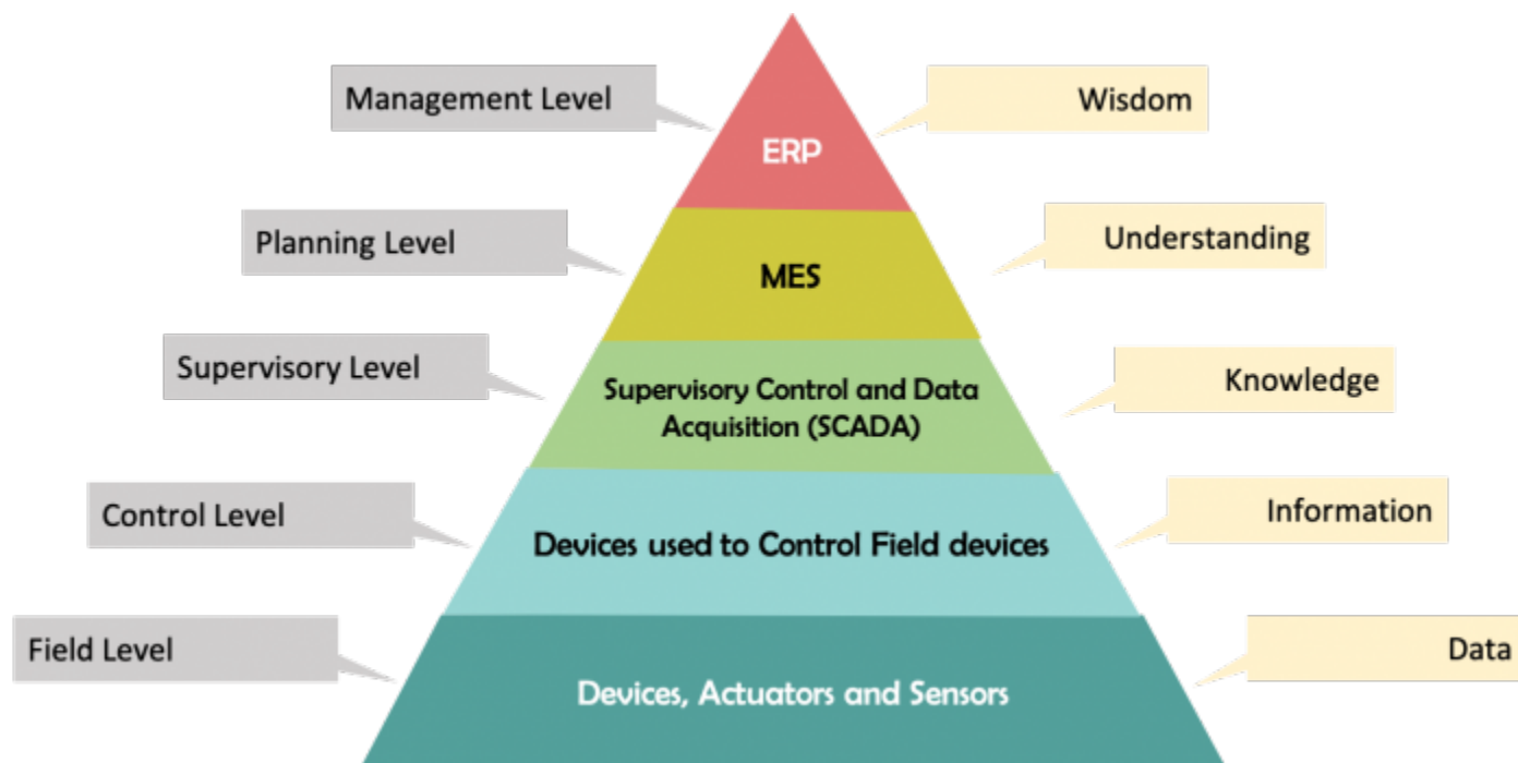
Figure 1: Automation Pyramid
