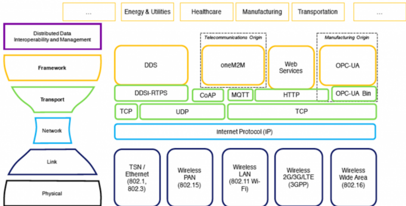
Figure 1: The Industrial Internet Consortium's Connectivity Framework layer provides the foundation for the interoperable transfer of common structured data across systems and domains 7)
