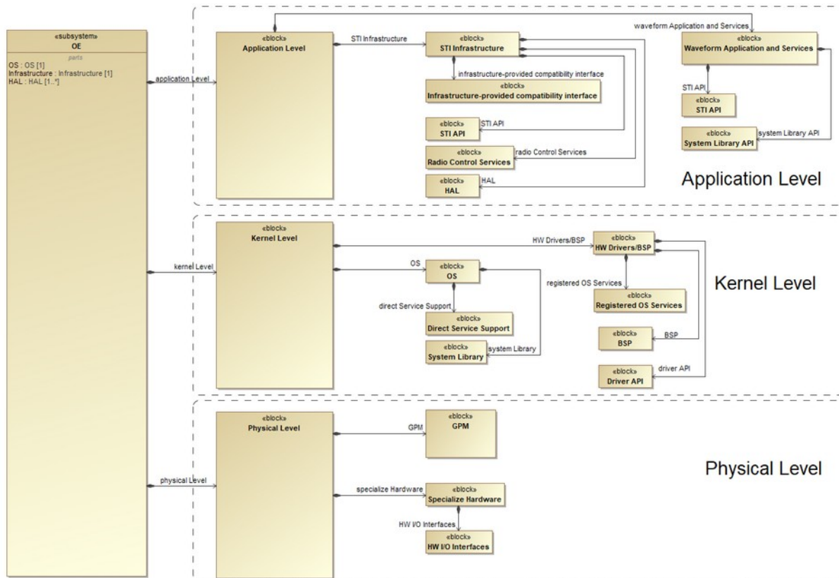
Figure 11: Operating Environment
