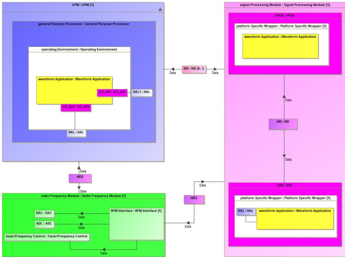
Figure 8: Notional High Level Software and Configurable Hardware Design
