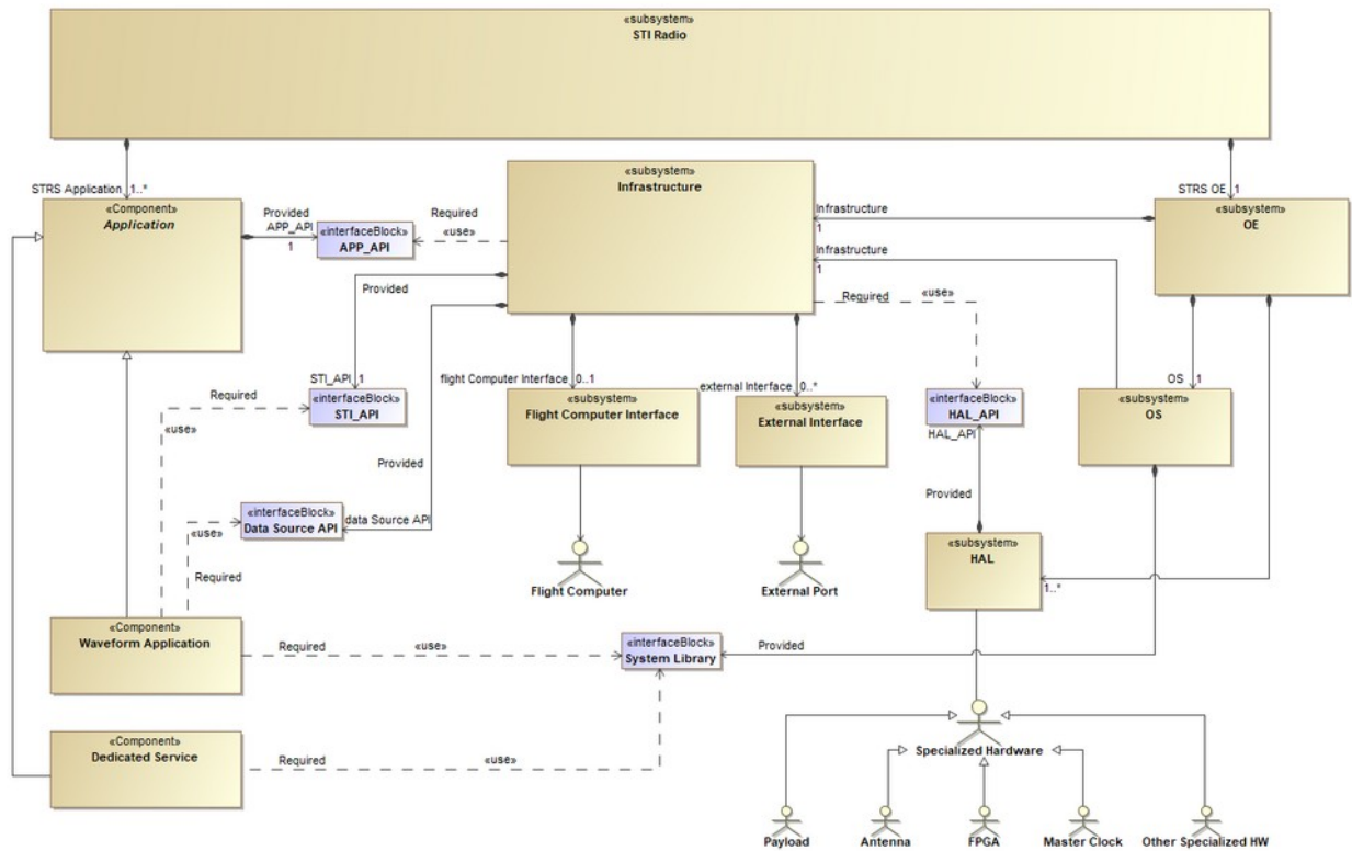
Figure 10: Layered Structure
